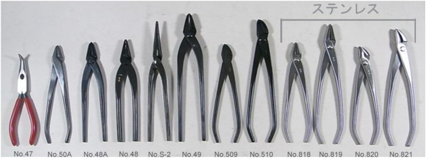
No.47 No.50A No.48A No.48 No.S-2 No.49 No.509 No.510 No.818 No.819 No.820 No.821 170mm 175mm 180mm 180mm 210mm 230mm 170mm 220mm 180mm 215mm 175mm 200mm
